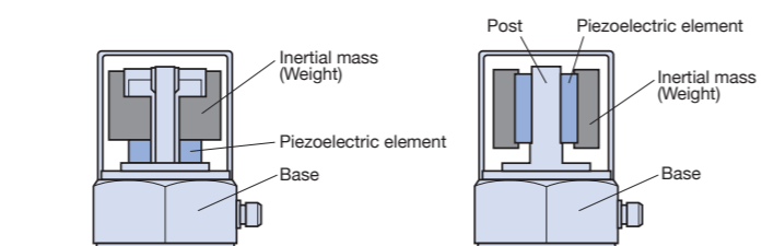
(a) Compressed type • Robust against impact force
