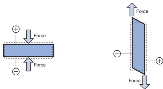
An electric charge is generated when either a compressing force or a pulling force is applied to the piezoelectric element in the axial direction.
