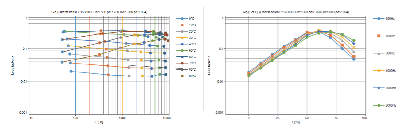
Loss factor of damping material alone
