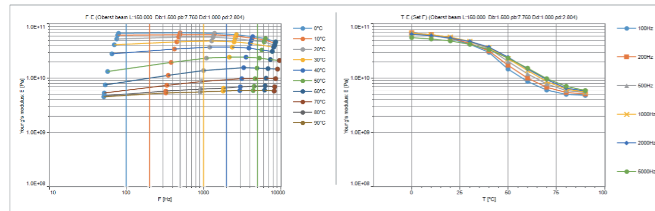
Young's modulus of damping material alone
