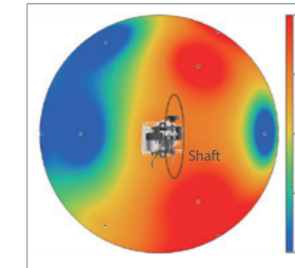
Sound pressure level distribution (5 kHz)
