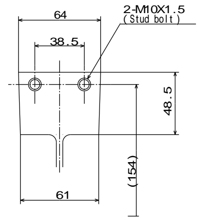
Bolt attachment position (Viewed from direction B)
