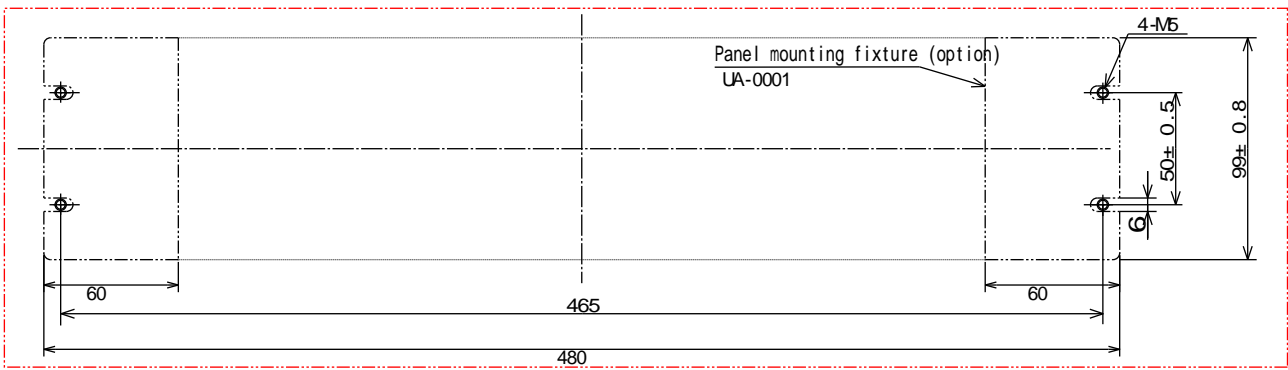
When mounting the 480mm width rack
