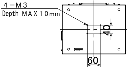
Rear view (1 : 5)
