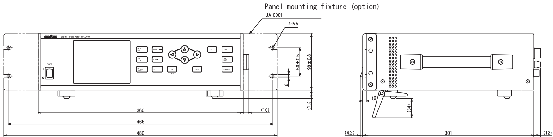
When mounting 480mm width rack
