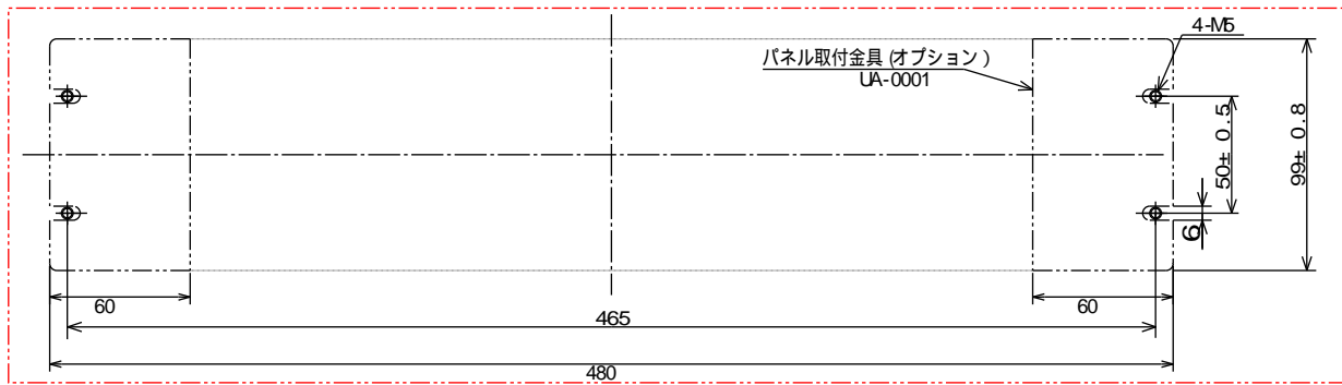
When mounting 480mm width rack
