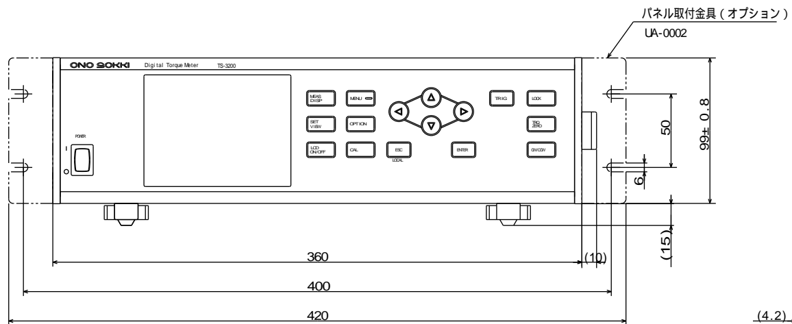
When mounting 480mm width rack
