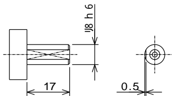
Shaft-end detail dimension
