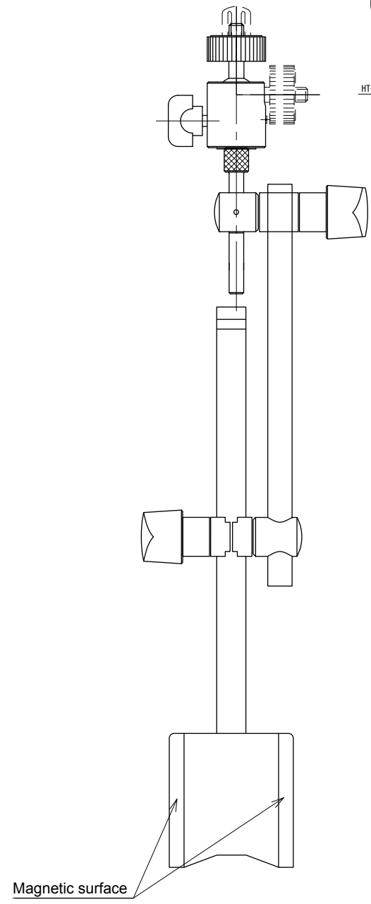
Assembling image of HT-0521A and HT-0522
