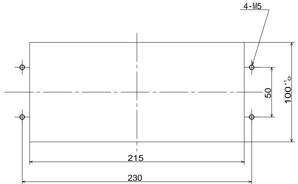
Panel cutout dimensions
