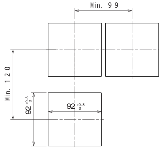
PANEL-CUT DIMENSIONS
