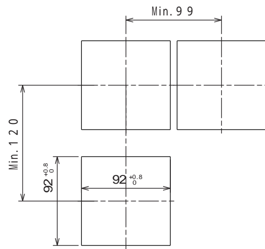
PANEL-CUT DIMENSIONS
