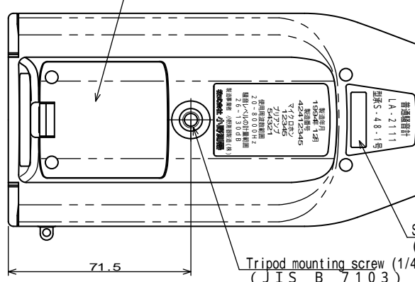
Battery compartment lid (4 AA-type batteries)
