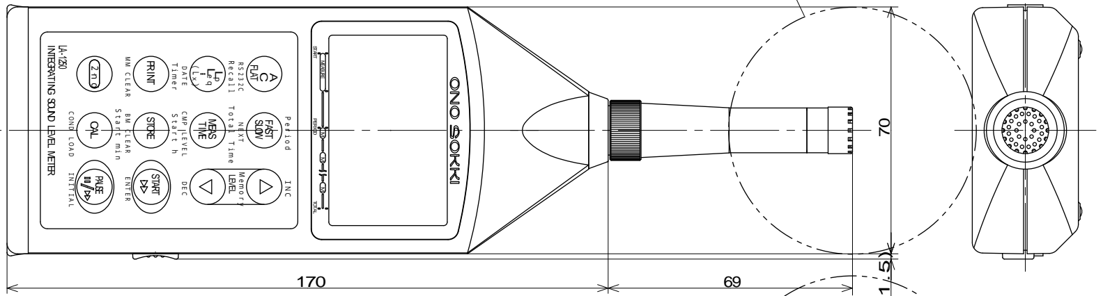
Windscreen Ø 70
