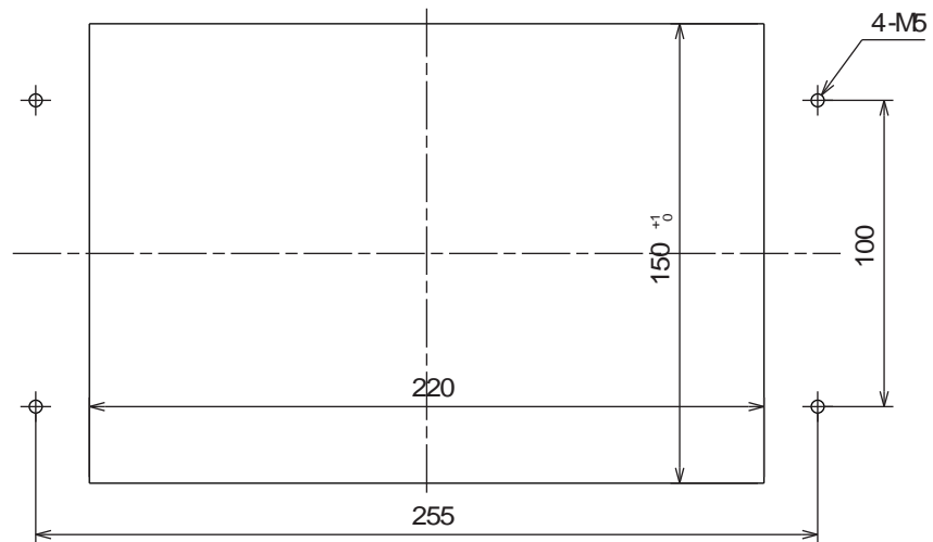
PANEL-CUT DIMENSIONS
