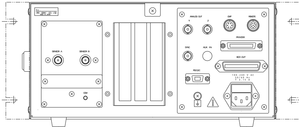
REAR VIEW
