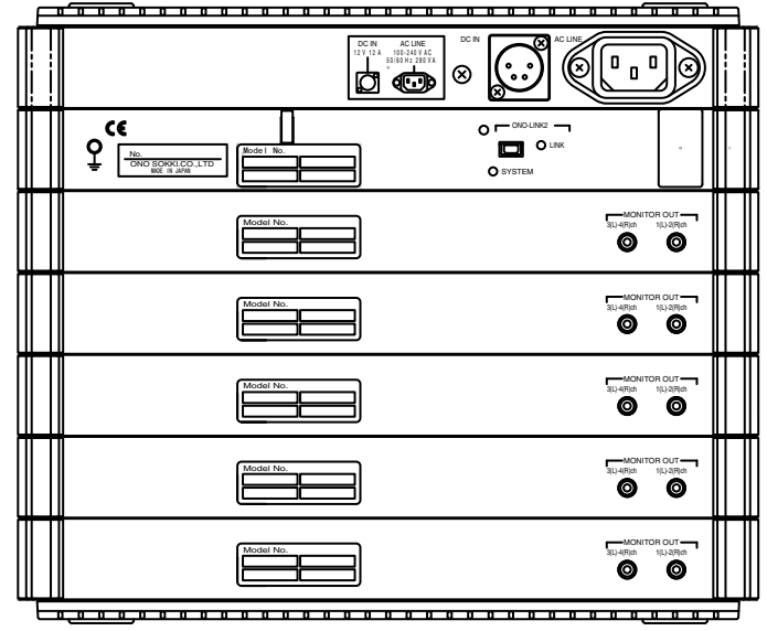
REAR VIEW 20-channel basic unit for the DS-2000 DS-2100+DS-0290+DS-0264 X 5 (DS-2120)
